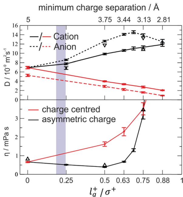
Fig. 16 Diffusion and viscosity as a function of charge separation. The blue shaded area indicates the l_q^+/\sigma^+ range for the [C_4C_{1im}]^+ cation. The charge centred systems where charge separation is achieved by decreasing the size are shown in red. Reprinted (adapted) from H. V. Spohr and G. N. Patey, J. Chem. Phys. , 2009, 130 , 104506, with the permission of AIP Publishing. 217
