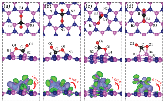
Fig. 13 Top and side views of the most energetically favorable configurations of adsorbed \text{CO}_2 on the dh -BN with (a) V_N , (b) V_B , (c) SW, and (d) B_N . The magenta, blue, black and red balls represent the B, N, C, and O atoms, respectively. The top and middle panel shows the top and side views, respectively. Bottom: The corresponding side views of the geometric structures with the charge density difference plot. The green and violet isosurfaces with iso-value of \pm 0.003 \text{ e} \text{ \AA}^{-3} , represent the accumulation and depletion of electron, respectively. The red arrow shows the electron transfer in direction and value.
