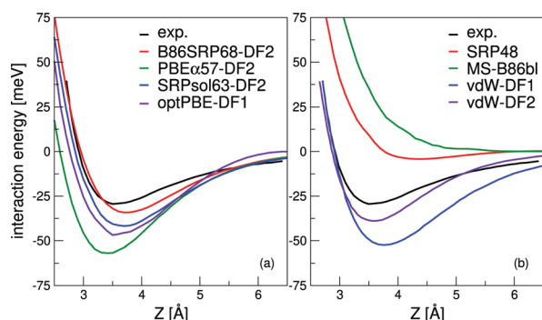
Fig. 3 The computed interaction energy of H 2 parallel to the Cu(111) surface above a top site ( \phi = 0^\circ, \theta = 90^\circ ) is compared with experimental results 59 (black). Panel (a) shows the calculated van der Waals well for the B86SRP68-DF2 (red), PBE \alpha 57-DF2, SRPsol63-DF2 and optPBE-DF1 41 DFs, and panel (b) for the SRP48, 10 MS-B86bl, 12 vdW-DF1 96 and vdW-DF2 97 DFs.
