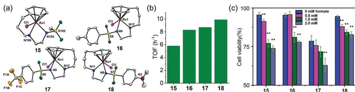
Fig. 8 (a) ORTEP diagrams of the X-ray crystal structures of tethered Ru II catalysts 15–18 with sulfonyl substituents on the diamine. Figure reproduced from ref. 23; F. Chen et al. , Organometallics 2018, 37 , 1555, published by The American Chemical Society. (b) TOFs for complexes 15–18 for NAD + reduction in MeOH-d 4 /D 2 O (1:9 v/v) determined by UV-vis spectroscopy (final concentrations: Ru complex 28 μM, NAD + 170 μM, NaHCO 2 34 mM, molar ratio 1/6/1200). 23 (c) Cell viability of A2780 cancer cells when incubated with complexes 15–18 (at equipotent 1/3 × IC 50 concentrations) and various sodium formate concentrations (0, 0.5, 1.0, and 2.0 mM) for 24 h. The figure is reproduced from ref. 23; F. Chen et al. , Organometallics 2018, 37 , 1555, published by The American Chemical Society.
