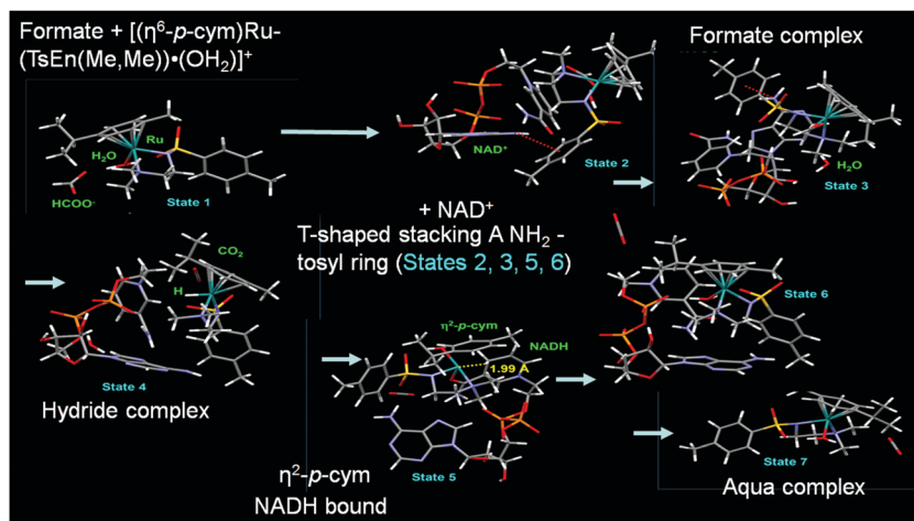
Fig. 7 Catalytic cycle for NAD + reduction by the complexes 9–14 based on DFT modelling. Reproduced from ref. 22; F. Chen et al. , Dalton. Trans. , 2018, 47 , 7178, published by The Royal Society of Chemistry.
