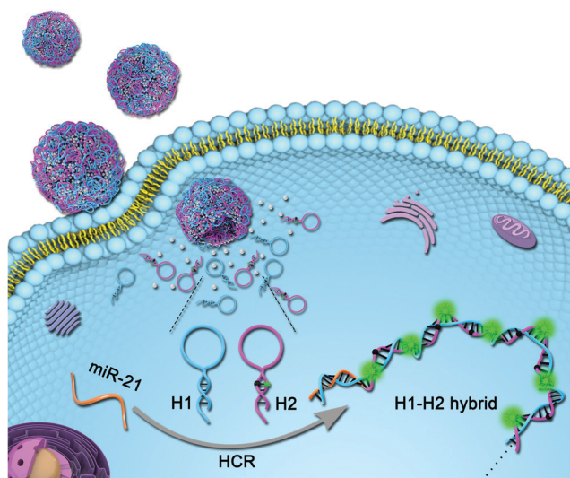
Scheme 2 Schematic illustration of imaging of miR-21 in living cells based on NWs. Herein the FAM and BHQ1 fluorophores are represented by green colored polygons and black colored spheres, respectively.
