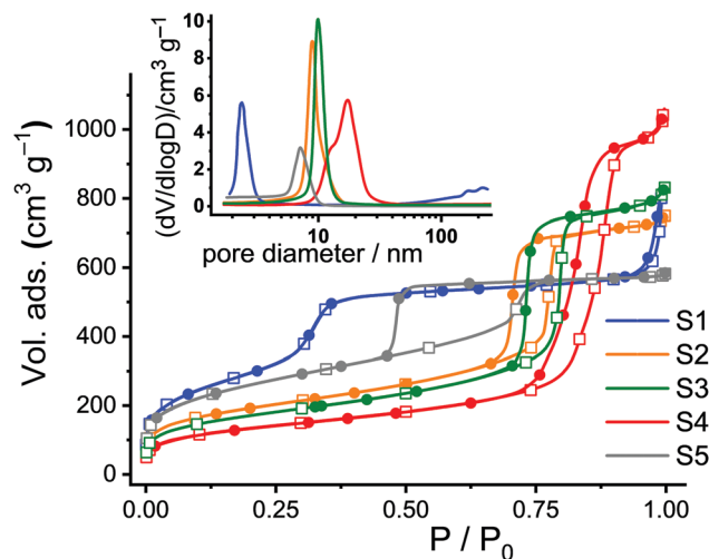
Fig. 2 Adsorption (hollow squares) and desorption (solid circles) isotherms for calculated S1–S5 . Inset: Corresponding pore size distributions.
