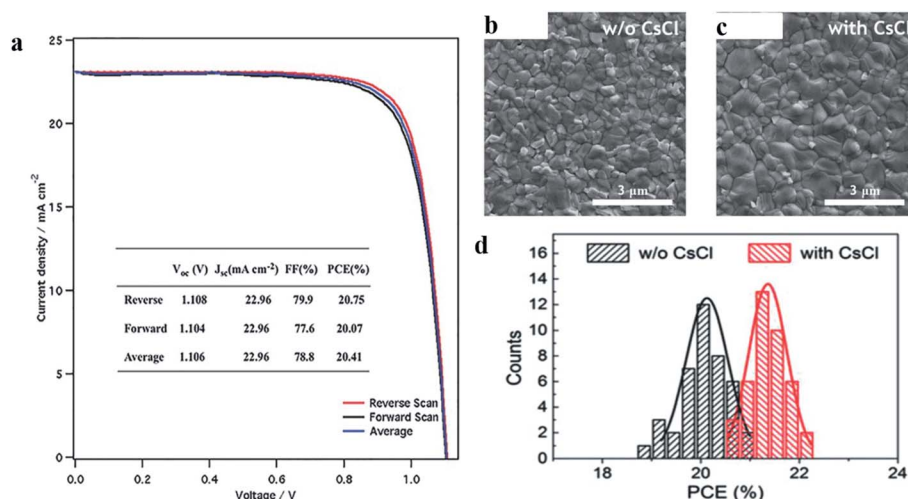
Fig. 20 (a) J-V curves of best performing perovskite solar cell devices. Reproduced by permission ref. 131, Copyright 2016 Wiley-VCH Verlag GmbH & Co. KGaA, Weinheim. Scanning electron microscope top-view image of perovskite film fabricated by (b) PSG method and (c) CsCl-enhanced \text{PbI}_2 precursor method. (d) Histogram of solar cell efficiencies with Gaussian function fitting in reverse scan for 40 devices. The black curve is for without CsCl and the red curve is for with CsCl in eight batches. Reproduced by permission ref. 132, Copyright 2018 Wiley-VCH Verlag GmbH & Co. KGaA, Weinheim.
