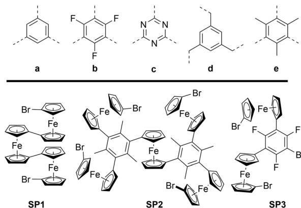
Scheme 1 (Top) Preparation of tris-phosphanes 1a-d and complexes [( 1a-c )E]. (I) Pd pre-catalyst, THF, r. t.; (II) n BuLi, Ph 2 PCL, THF, -80 °C to r. t.; (III) [E]-X ([E]-X = BH 3 ·SMe 2 or [AuCl(tht)]), CH 2 Cl 2 , r. t.; (Bottom) crystallographically characterised side products obtained during the syntheses of 4d (SP1), 4e (SP2), and 4b (SP3). For their solid-state structures, see Fig. S3.†
