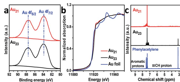
Fig. 5 (a) Au 4f XPS and (b) Au L 3 -edge XANES profiles of \text{Au}_{21}(-\text{SR})_{12}(\text{Ph}_2\text{PCH}_2\text{PPh}_2)_2 and \text{Au}_{23}(\text{SR})_{16} . (c) The 1 H NMR spectra of Au-acetylide species.
