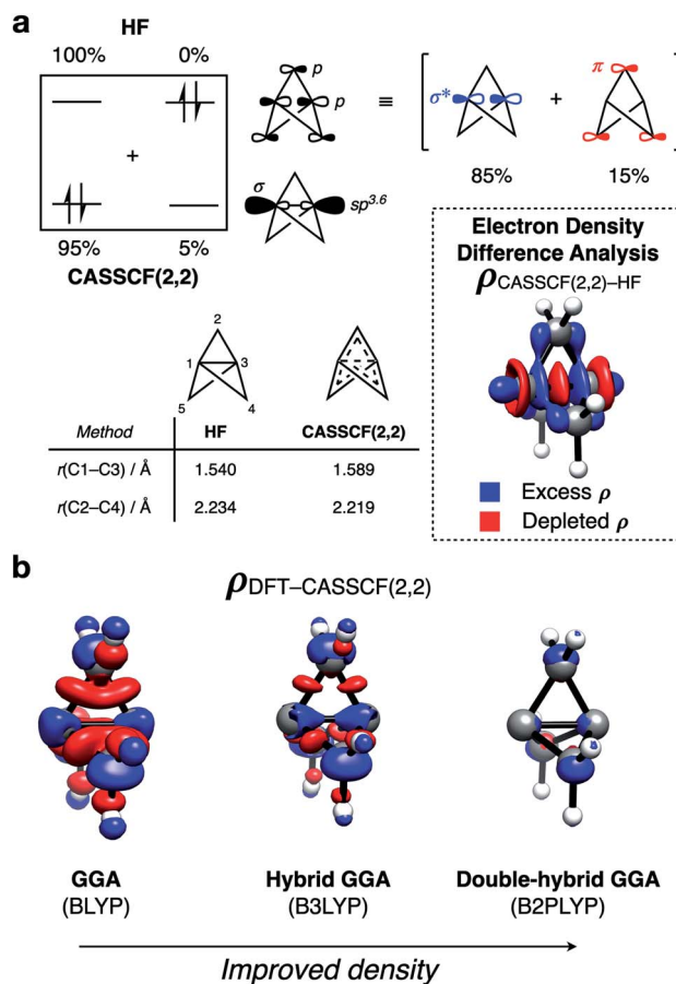
Fig. 2 (a) Top: populations and symmetries of MOs in the (2,2) active space with their corresponding atomic orbital composition. Bottom left: effect of \sigma-\pi -delocalization on key geometric features of 1 . Inset: [CASSCF(2,2)]–[RHF] electron density difference plot for 1 , isovalue = 0.002 a.u. (b) DFT electron density difference plot for 1 : [BLYP]–[CASSCF(2,2)] (left), [B3LYP]–[CASSCF(2,2)] (center), [B2PLYP]–[CASSCF(2,2)] (right); isovalue of 0.01 a.u. Geometry optimized at CASSCF(2,2). All calculations use the def2-QZVPP basis set.
