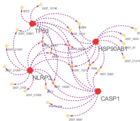
Fig. 3 Compound–target network.
