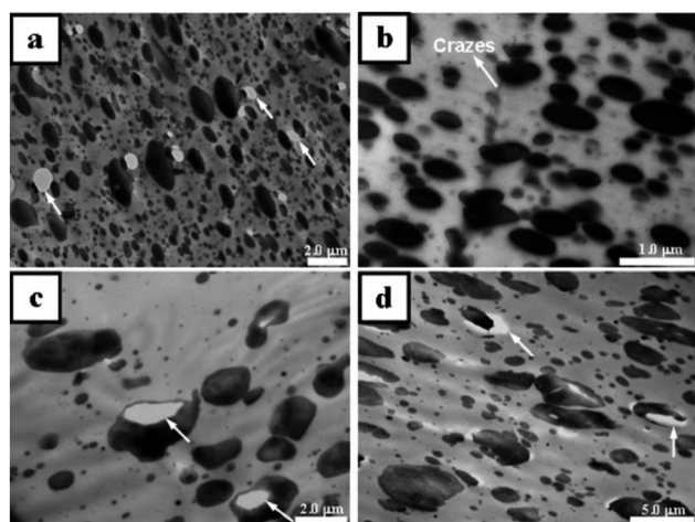
Fig. 23 TEM micrographs of stress-whitening zone: (a) PLA/EBA-GMA (80/20) binary blend, low-magnification (7500x); (b) PLA/EBA-GMA (80/20) binary blend, high magnification (30 000x) at the localized area; (c) PLA/EBA-GMA/EMAA-Zn (80/15/5) ternary blend; (d) PLA/EBA-GMA/EMAA-Zn (80/5/15) ternary blend. Ref. 150, copyright 2011. Reproduced with permission from American Chemical Society.
