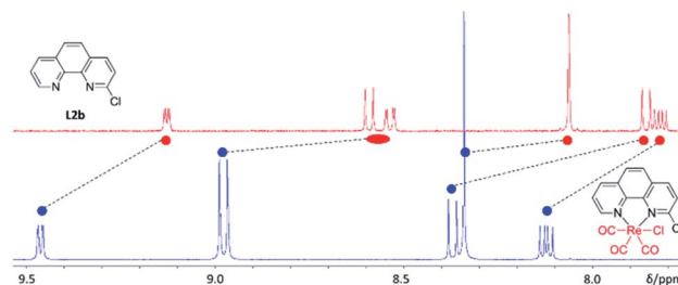
Fig. 6 Example of the downfield chemical shifts in ^1\text{H} -NMR aromatic signals observed when complexing L2b (top, red) with [\text{Re}(\text{CO})_5\text{Cl}] to form [\text{Re}(\text{L2b})(\text{CO})_3\text{Cl}] (bottom, blue). The shifts suggest electron withdrawal from the \pi -aromatic system which likely facilitates nucleophilic substitution for [ ^{18}\text{F} ]fluoride.
