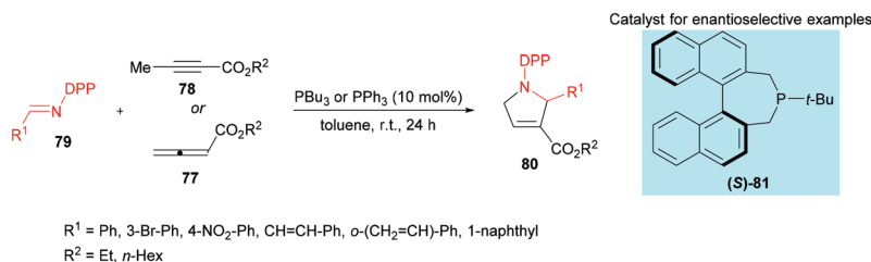
Scheme 18 Phosphine-catalyzed synthesis of pyrrolines from N -DPP-imines and allenoates/2-butynoates.
