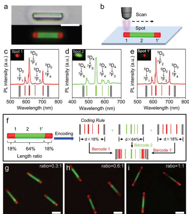
Fig. 8 (a) Bright-field and PL microscopy images of a segregated Ln-MOF heterostructure. Scale bar is 10\ \mu\text{m} . (b) Schematic illustration of a heterostructure excited with a focused laser beam. Each part (marked as 1, 2, 1') of the heterostructure was selectively excited with a CW laser beam ( 375\text{ nm} ). (c-e) Corresponding PL spectra collected from three different areas and the generated barcodes (marked as 1, 2, 1' shown in b). (f) Schematic illustration of the encoding strategy based on the segregated Ln-MOF heterostructure. According to the different block lengths in a heterostructure, the as-designed barcodes were compressed with the corresponding length ratio, which can be defined as the sub-barcodes. The barcode was subsequently generated by combining the three parts of the sub-barcodes. (g-i) PL images of the segmented structure with various block lengths. The block length can be precisely controlled by adjusting the epitaxy precursor-to-seed ratio in the reaction system. Scale bars are 10\ \mu\text{m} . Reproduced with permission from ref. 42. Copyright 2019, Wiley-VCH.
