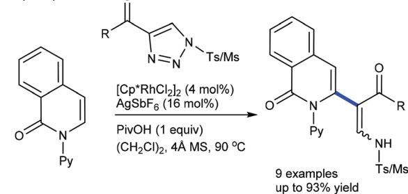
Scheme 31 Coupling of isoquinolones with 4-acyl-1-sulfonyl triazoles.
