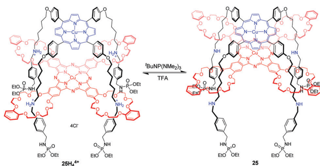
Fig. 25 Tanaka's molecular elevator.
