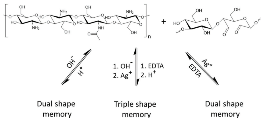
Fig. 8 Schiff base bonds in the triple shape memory gel hydrogel reported by Chen and co-workers respond to pH and Ag^+ ions. 138
