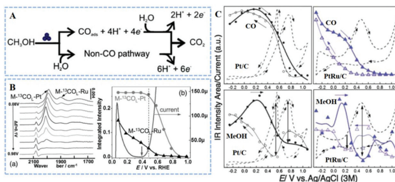
Fig. 1 (A) MOR reaction pathways. Reproduced with permission from ref. 81. Copyright 2006, American Chemical Society. (B) In situ ATR-SEIRAS of preadsorbed M- 13 CO L on the Ru/Pt (M- 13 CO L refers to the linearly bonded CO generated by methanol), and the integrated IR intensity of the M- 13 CO L -Pt and M- 13 CO L -Ru as a function of electrode potential. Reproduced with permission from ref. 82. Copyright 2015, John Wiley & Sons Ltd. (C) CO ads and CH 3 OH ads band integrals as a function of potential in both positive and negative scans on Pt/C and PtRu/C, respectively. Reproduced with permission from ref. 84. Copyright 2012, Royal Society of Chemistry.
