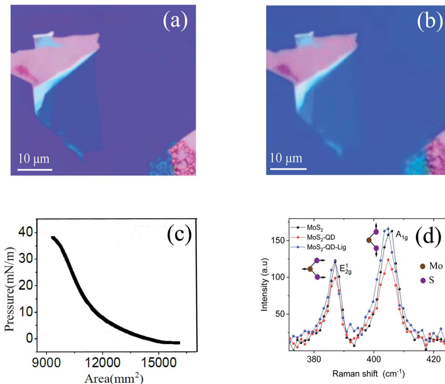
Fig. 2 (a) Optical image of monolayer \text{MoS}_2 . (b) The optical images of the \text{MoS}_2 -QD hetero-structure after transferring the compact monolayer of the QD film using the Langmuir-Blodgett (LB) technique, with the dot-dot separation, \delta and the \text{MoS}_2 -QD separation, d , being controlled through chemical methods. (c) The surface pressure vs. area (isotherm) curve of LB for the QD monolayer; the film was transferred at a surface pressure of 35 \text{ mN m}^{-1} . (d) The Raman spectra of \text{MoS}_2 , \text{MoS}_2 -QDs, and \text{MoS}_2 -QDs after ligand exchange.
