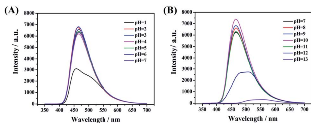
Fig. 8 Fluorescence spectra of CDs-3 with varying pH including (A) acid solution (pH = 1–7) and (B) basic solution (pH = 7–13).
