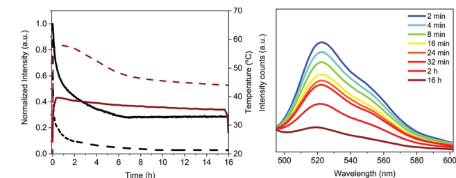
Fig. 5 Typical performance of 'on-chip' Bio-HLEDs operating at high-applied currents of 200 mA. Left: Overall emission intensity decay (black) along with the temperature changes (red) over time for Bio-HLEDs with FP-SF (solid line) and FP-polymer (dashed line). Right: Electroluminescence spectra of Bio-HLEDs with FP-SF phosphors over time.
