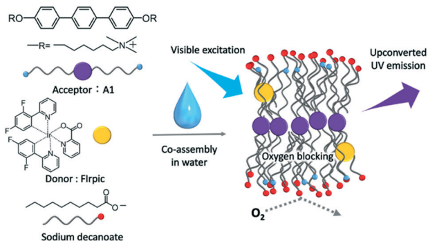
Fig. 1 Schematic illustration of the supramolecular system for air-stable aqueous vis-to-UV TTA-UC. Cationic acceptor A1 , donor Firpic, and anionic sodium decanoate (Dec) form aqueous co-assemblies with oxygen blocking ability.
