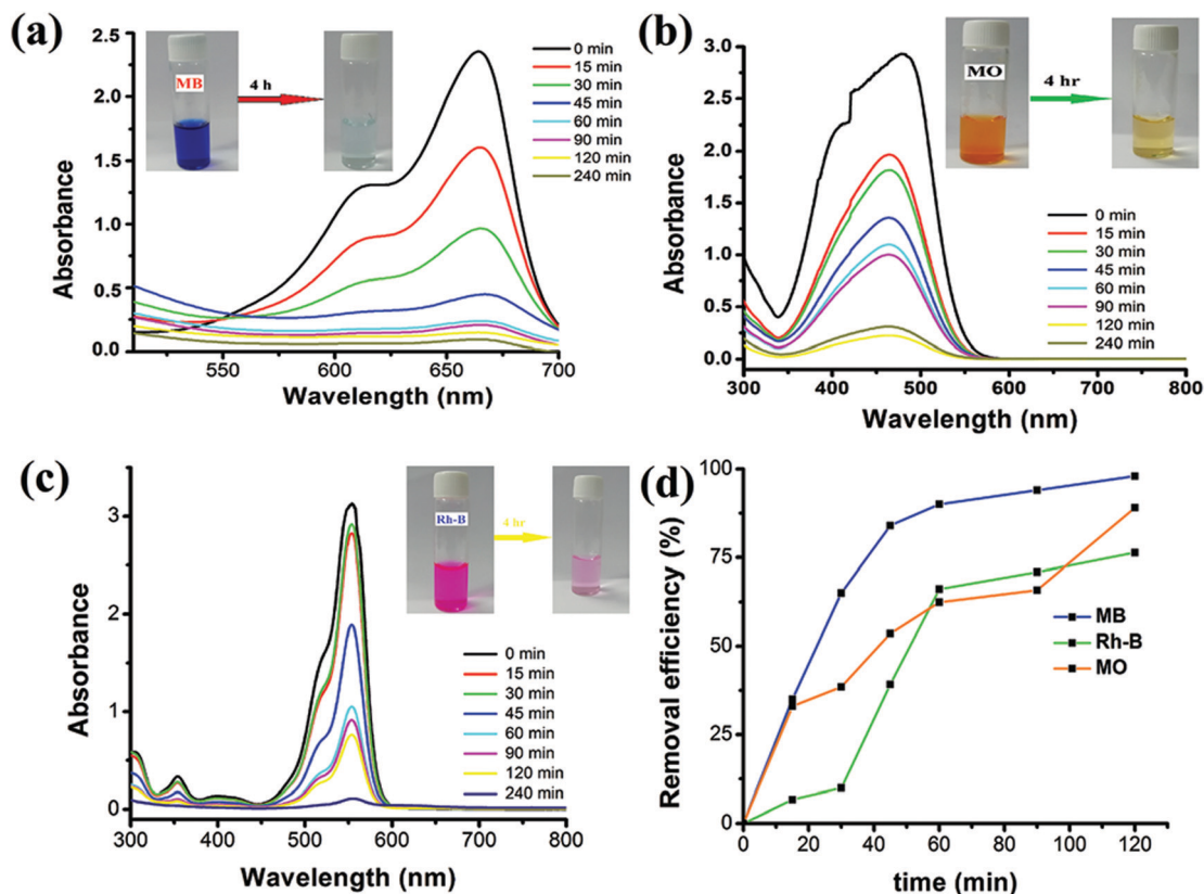
Fig. 15 Change in absorption spectrum of CP ( 1 ) in the presence of different dyes: MB (a), MO (b), and Rh-B (c) at different time intervals and (d) efficiency of CP ( 1 ) to remove different dyes. 250 Reproduced from ref. 250 with permission from the Royal Society of Chemistry.
