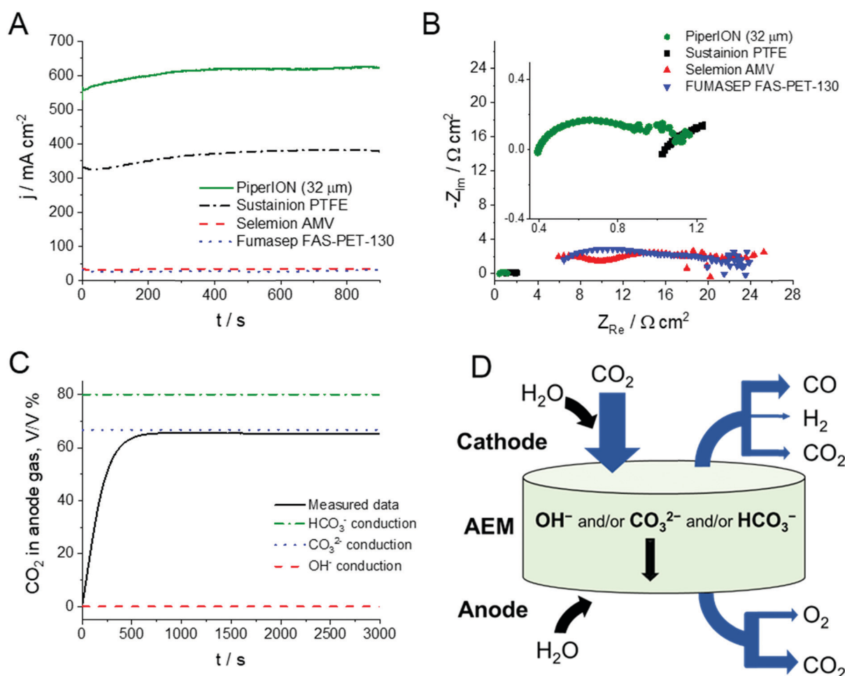
Fig. 4 (A) Chronoamperometric curves and (B) EIS traces of electrolyzers assembled with different commercial membranes, operated with T = 60^\circ\text{C} , 0.1\text{ mol dm}^{-3} CsOH anolyte, \Delta U = 3.0\text{ V} , with u = 12.5\text{ cm}^3\text{ min}^{-1}\text{ cm}^{-2} \text{CO}_2 feed rate. (C) A representative anode gas analysis curve recorded during chronoamperometric measurements shown in Fig. 3. (D) Illustration of the mass balance of the electrolysis process, where the width of the blue arrows is proportional to the magnitude of the different fluxes at 40% conversion, while the black arrows only indicate the directions of the different fluxes.
