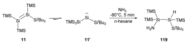
Scheme 46 Activation of NH 3 by tetrasilyldisilene 11 and bis(silyl)silylene 11' .
