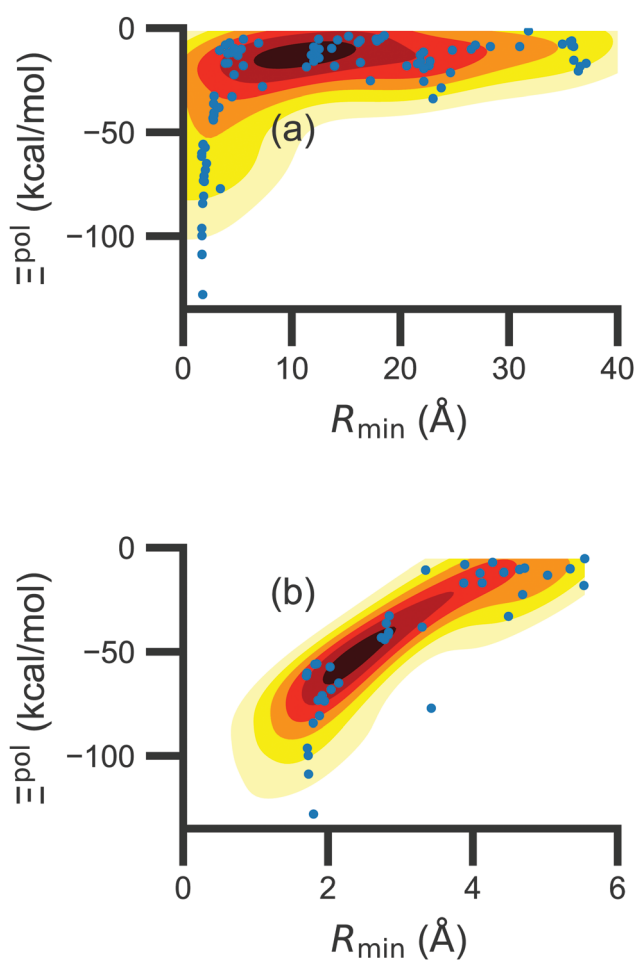
Fig. 3 Scatter plot of the ligand polarization energy \bar{\epsilon}^{\text{pol}} as a function of the minimum distance between a ligand and cation atom, R_{\text{min}} , for (a) the entire range of R_{\text{min}} and (b) R_{\text{min}} < 6 Å.
