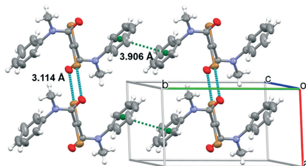
Fig. 3 Crystal packing of 1 showing the Br⋯O halogen bonds and distances between rings' centroids (cyan and green dashed lines, respectively). Ellipsoids drawn at 50% probability.
