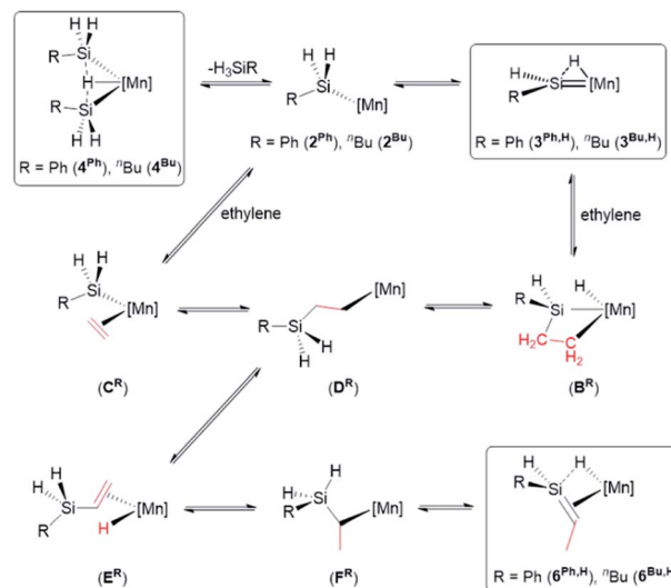
Scheme 6 Proposed pathways for reactions of disilyl hydride complexes [(dmpe) 2 MnH(SiH 2 R) 2 ] ( 4 Ph ; R = Ph, 4 Bu ; R = t Bu) with ethylene to form silene hydride complexes [(dmpe) 2 MnH(RHSi=CHMe)] ( 6 Ph,H ; R = Ph, 6 Bu,H ; R = t Bu). [Mn] = Mn(dmpe) 2 . Only one isomer of 3 R,H is shown. Boxes indicate complexes which have been isolated or spectroscopically observed.
