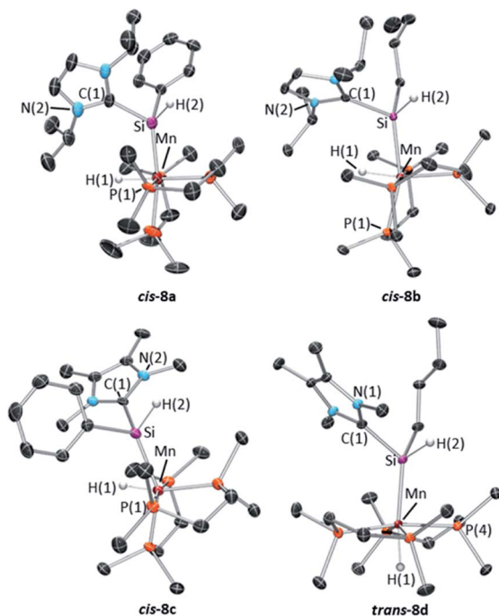
Fig. 8 X-ray crystal structures of (top left) cis -[(dmpe) 2 MnH(=SiHPh) (iPr) NHC)] ( cis - 8a ), (top right) cis -[(dmpe) 2 MnH(=SiH t Bu) (iPr) NHC)] ( cis - 8b ), (bottom left) cis -[(dmpe) 2 MnH(=SiHPh) (Me) NHC)] ( cis - 8c ), and (bottom right) trans -[(dmpe) 2 MnH(=SiH t Bu) (Me) NHC)] ( trans - 8d ) with ellipsoids drawn at 50% probability. Most hydrogen atoms have been omitted for clarity. In the case of 8a–b , the structures exhibit some disorder, and only the dominant conformation is shown.
