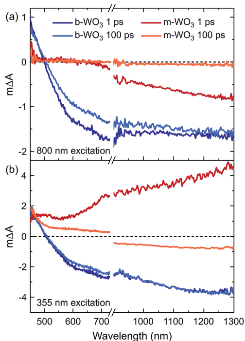
Fig. 4 Transient absorption spectra of m- WO_3 and b- WO_3 for excitation wavelengths of (a) 800 nm and (b) 355 nm. For each sample and excitation wavelength, spectra probed at 1 ps and 100 ps after excitation are shown. All spectra were acquired at an excitation intensity of 0.26 \text{ mJ cm}^{-2} under argon atmosphere.
