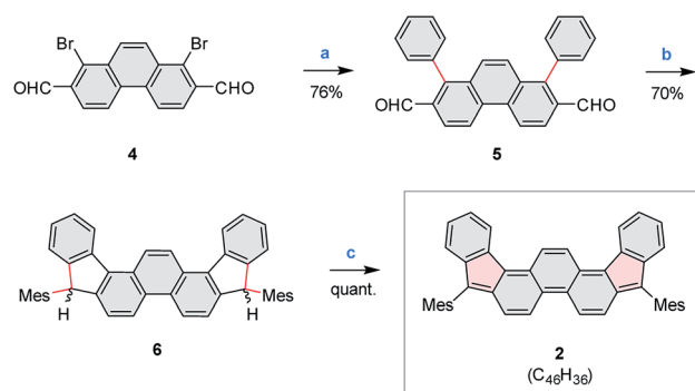
Scheme 2 Synthesis of 5,10-dimesityldiindeno[1,2- a :2',1'- f ]phenanthrene ( 2 ). Reagents and conditions: (a) PhB(OH) 2 , Pd(PPh 3 ) 4 , Na 2 CO 3 (aq), dioxane, reflux, overnight. (b) (1) MesMgBr, THF, rt, overnight. (2) BF 3 ·Et 2 O, DCM, rt, 10 min. (c) 2.5 equiv. DDQ, toluene, rt, overnight.
