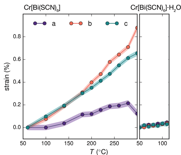
Fig. 4 Crystallographic strain of \text{Cr[Bi(SCN)}_6\text{]} and \text{Cr[Bi(SCN)}_6\text{]}\cdot\text{H}_2\text{O} along the unit cell axes determined via variable temperature powder X-ray diffraction. The total change in volume for \text{Cr[Bi(SCN)}_6\text{]} over this region (1.7%) is significantly smaller than the volume difference between the hypothetical aristotype and the room temperature structure (54%). As the changes in \sin(\theta) are two orders of magnitude smaller than the strains along the unit cell axis directions the strain eigenvalues are to a good approximation equal to the unit cell axis strains.
