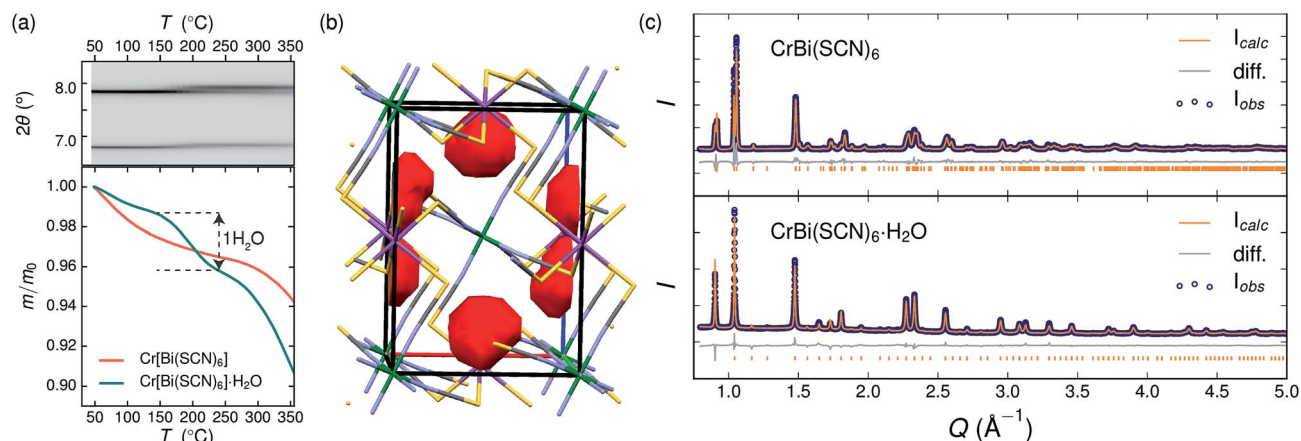
Fig. 3 (a) Dehydration of \text{Cr[Bi(SCN)}_6\text{]}\cdot\text{H}_2\text{O} between 150 °C and 200 °C. Top panel: variable temperature PXRD measurements of \text{Cr[Bi(SCN)}_6\text{]}\cdot\text{H}_2\text{O} , highlighting the separation of the \{110\} and (002) reflections at around 2\theta = 7.8^\circ . Bottom panel: TGA measurements on hydrated (teal) and anhydrous (orange) show the presence of a step at around 170 °C in the hydrated sample, but no similar step in the dehydrated sample. (b) Structure of \text{Cr[Bi(SCN)}_6\text{]}\cdot\text{H}_2\text{O} determined from powder diffraction data, with guests removed. The void space within the cell is shown in red (contact surface determined using Mercury, probe size 1.2 Å). Colour scheme as follows: Bi, purple; Cr, green; N, blue; C, black and S, yellow. (c) Rietveld refinement of synchrotron powder diffraction data for both hydrated and anhydrous \text{Cr[Bi(SCN)}_6\text{]} .
