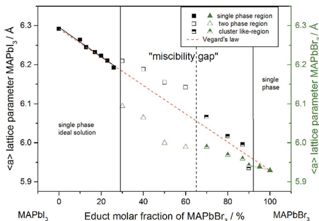
Fig. 2 Room temperature cubic mean lattice parameter \langle a \rangle of \text{MAPb(I}_{1-x}\text{Br}_x)_3 solid solutions and Vegard derived linear interpolation of cubic lattice parameters (dashed): lattice parameters of the iodine rich part follow Vegard's law whereas lattice parameters in the two-phase region do not show a linear trend. The miscibility gap is divided into two regions: empty squares and triangles corresponding to clearly resolved iodine rich and bromine rich peaks, half-filled squares and triangles corresponding to bromine rich peaks with iodine cluster-like regions.
