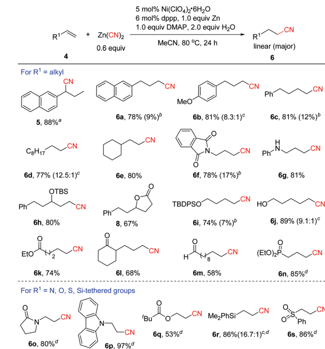
Scheme 3 Scope of aliphatic alkenes. Isolated yields. a 5 mol% NiCl 2 ·6H 2 O, 6 mol% Xantphos, 20 mol% Zn, dioxane/H 2 O = 50/1. b The yields of the branched nitrile 7 are shown in parentheses. c Overall yields of 6 and 7 , and the ratio of 6 : 7 is shown in parentheses. d 5 mol% NiCl 2 ·6H 2 O, 6 mol% dpfp, 20 mol% Zn and 2.0 equiv. H 2 O were used in MeCN at 80 °C for 12 h.
