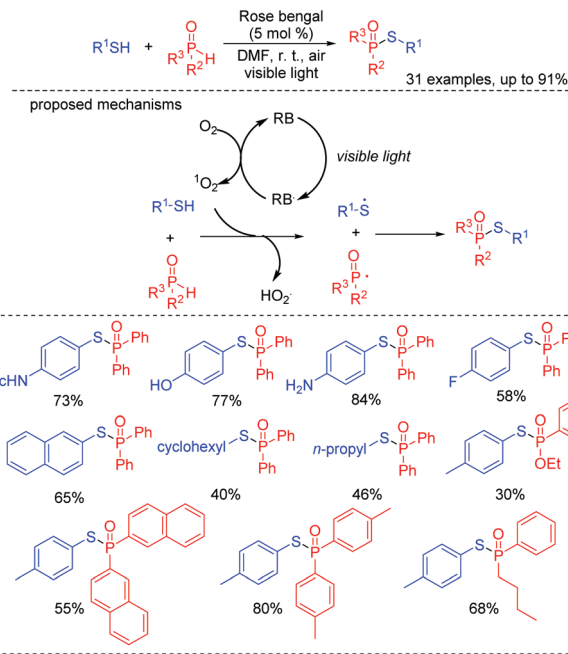
Scheme 24 Construction of S–P(O) bonds.
