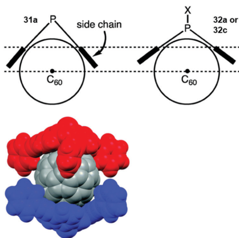
Fig. 43 Top: Illustration of the coordination of a P-centered triangulene with a deep ( 31a ) and a shallow bowl ( 32a/c ) to C_{60} . Bottom: Space-filling model of the ( P )- 31a \supset C_{60} complex. 20 Figure reproduced with kind permission; © 2015 The Royal Chemical Society.
