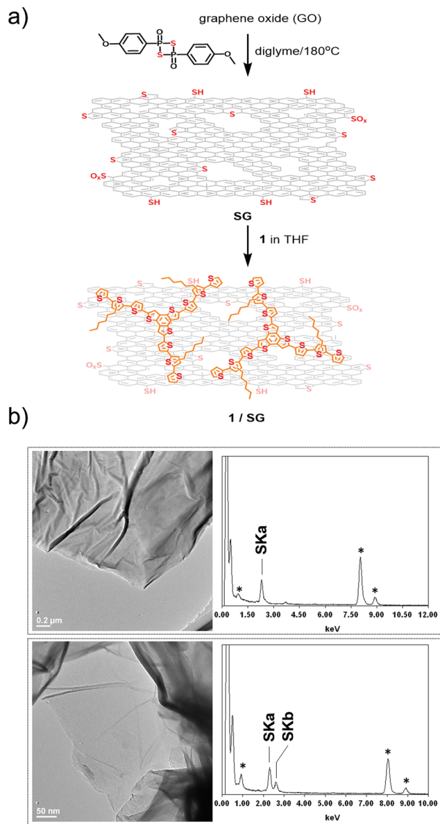
Fig. 1 (a) Preparation of the 1/S-G ensemble featuring oligothiophene 1 immobilized onto S-doped graphene via \pi - \pi interactions. (b) Representative HR-TEM images and EDX analysis of SG (upper panel) and 1/S-G (lower panel). With asterisks are marked EDX signals from the copper mesh grid.
