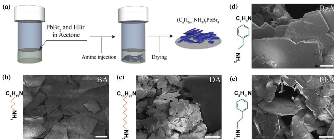
Fig. 1 (a) Schematic diagram of the facile fabrication process of the layered perovskite by injecting a primary amine to a mixture of \text{PbBr}_2 in \text{HBr} and acetone. (b–e) SEM images of the produced platelets when using short and long aliphatic molecules, such as butylammonium (BA) (b) and decylammonium (DA) (c), and aromatic ones as benzylammonium (BzA) (d) and phenethylammonium (PEA) (e). Scale bars: 100 \mu\text{m} .
