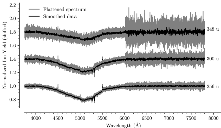
Fig. 7 Absorption spectrum in the range from 3750 Å to 7750 Å of C_{20}H_{10}D^+ complexed with 1, 12, and 24 He/ D_2 atoms/molecules, respectively. The flattened raw spectrum is shown in gray and is overlaid with a spectrum where the data has been smoothed (moving average over 10 nearest neighbors) for easier viewing. A broad absorption feature is observed between 4000 Å to 6000 Å together with two narrow lines near 5280 Å and 5320 Å. The positions of the latter do not shift as a function of the solvation and are caused by an increased output from our laser that we have not been able to fully correct for. The measurements at wavelengths above 6000 Å were performed with shorter dwell times and have a higher signal-to-noise ratio than those at shorter wavelengths. A small discontinuity is also visible where two datasets were spliced together at 5500 Å.
