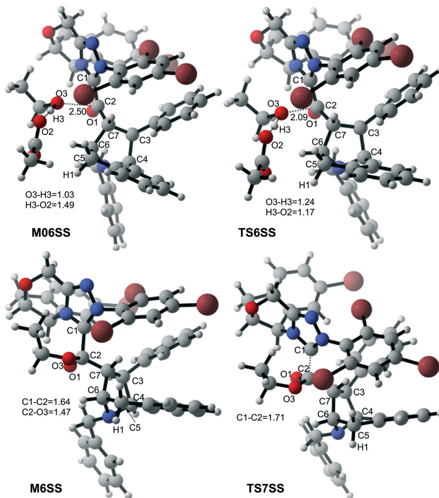
Fig. 4 3D-structures of the key transition states involved in stage 3 (distance in Å).
