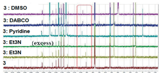
Fig. 11 ^{13}\text{C} NMR spectra of 3 in presence of different XB acceptors as deuterated solvents or dissolved in \text{CDCl}_3 .
