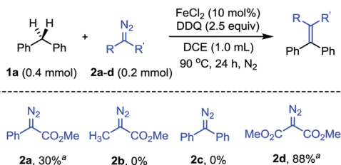
Scheme 2 Evaluation of the compatibility of diazo compounds.
