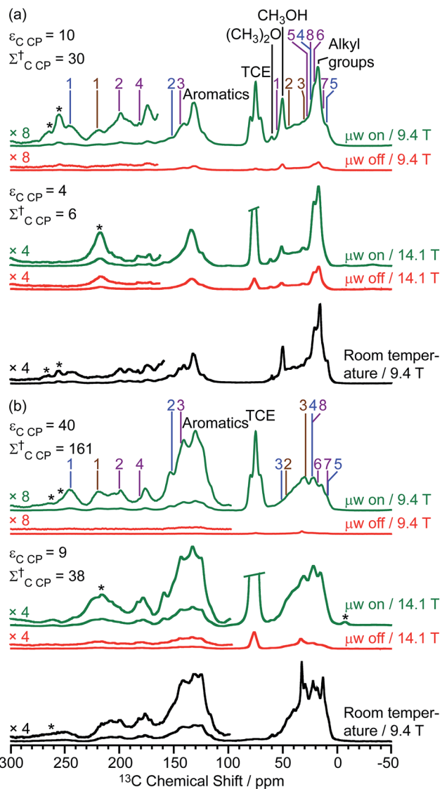
Fig. 3 ^{13}\text{C} CP MAS DNP spectra at 9.4 T, 110 K and 14.1 T, 125 K and room temperature experiments at 9.4 T of (a) activated M- \beta and (b) activated MMM- \beta . The assignments of the different carbocations (except methylnaphthalenium ions IV for clarity) are given with the same colors as their structures in Fig. 2. The experimental times for the spectra of activated M- \beta are \approx 7 minutes at 9.4 T DNP, \approx 9 minutes at 14.1 T DNP and \approx 52 minutes at room temperature at 9.4 T without DNP while for activated MMM- \beta they are \approx 2 minutes at 9.4 T DNP, \approx 6 minutes at 14.1 T DNP and \approx 1036 minutes at room temperature at 9.4 T without DNP. \Sigma^{\dagger} refers to the overall DNP gain and is calculated by comparing the DNP data to room temperature 9.4 T NMR spectra (see ESI ^{\dagger} ). All spectra were recorded at a MAS rate of 12.5 kHz with asterisks (*) denoting spinning sidebands.
