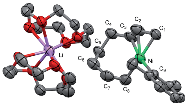
Fig. 2 An ORTEP drawing of one of the four asymmetric units of [\text{Ni}(\text{C}_8\text{H}_9)(\text{C}_8\text{H}_{12})_2] \cdot \text{Li}(\text{12-crown-4})_2(\text{thf})(\text{C}_5\text{H}_{12})_2 ( 8 ) with thermal ellipsoids at the 50% probability level. All hydrogen atoms and solvent molecules are omitted for clarity.
