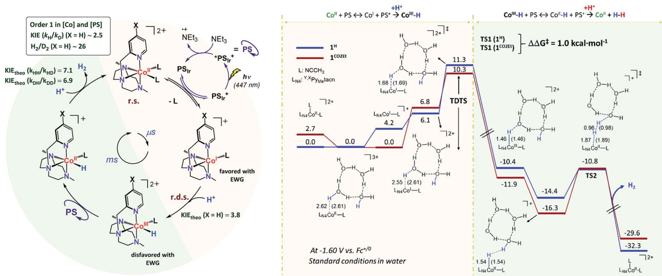
Fig. 11 (Left) Proposed mechanism for H_2 evolution catalysed by 1^R complexes. (Right) values are \Delta G . Energies are given in \text{kcal mol}^{-1} . B3LYP- D_3/\text{aug-cc-pVTZ}(-f)//\text{B3LYP-}D_3/6-31+G^* level of theory. Bond lengths for 1^H ( 1^{COEt} ) are shown in Armstrongs.
