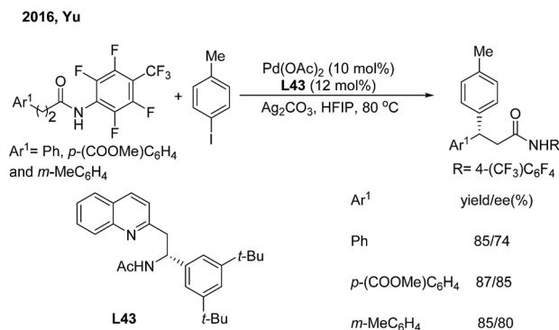
Scheme 30 Pd-catalyzed enantioselective \beta -arylation of aliphatic amides induced by chiral acetyl-protected aminoethyl quinoline ligands.
