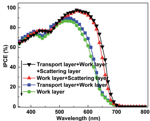
Fig. 8 IPCE patterns of devices with various photoanodes.
