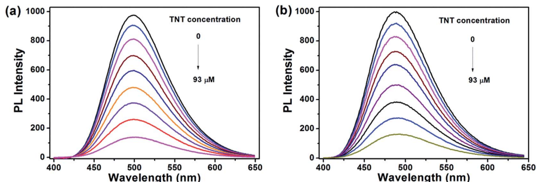
Fig. 3 PL spectra of (a) PTPA1-TPE and (b) PTPA2-TPE in 9 : 1 (v/v) water/THF solution containing different amounts of TNT. Polymer concentration: 10^{-5} M.
