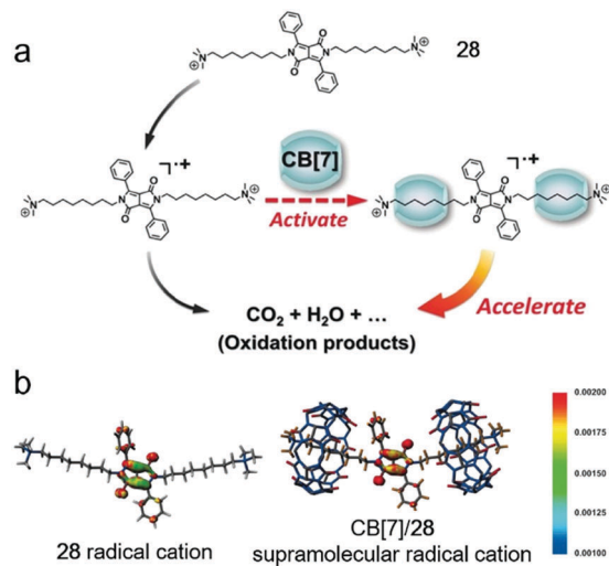
Fig. 20 (a) Schematic representation of CB[7] promoted Fenton oxidation. (b) Spin-density distribution of the 28 radical cation (left) and CB[7]/ 28 supramolecular radical cation (right). Adapted with permission from ref. 83. Copyright 2016 John Wiley and Sons.
