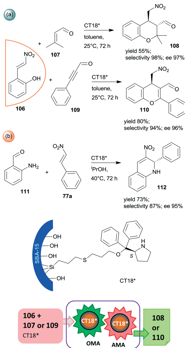
Scheme 31 Cascade oxa-Michael reaction (OMA) and asymmetric aza-Michael reaction and nitro-aldol condensation (b) catalysed by SBA-15 anchored diphenyl prolinol. 168
